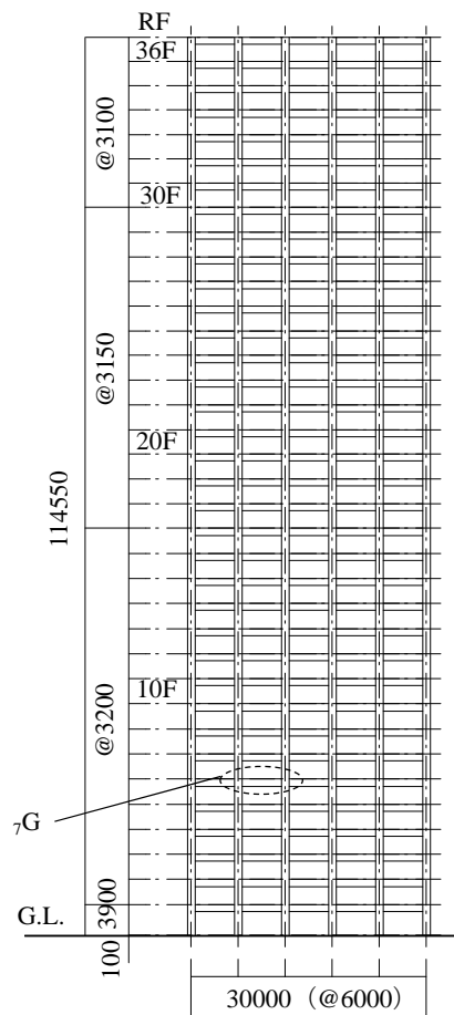
Figure 2. Frame elevation
