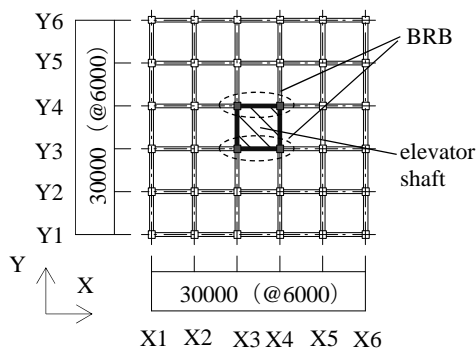
Figure 1. Frame plan
