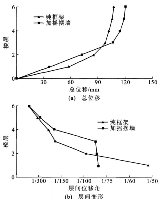
图10 模型1与模型3变形的比较 Fig.10 Comparisons on Drifts Between Model 1 and Model 3
